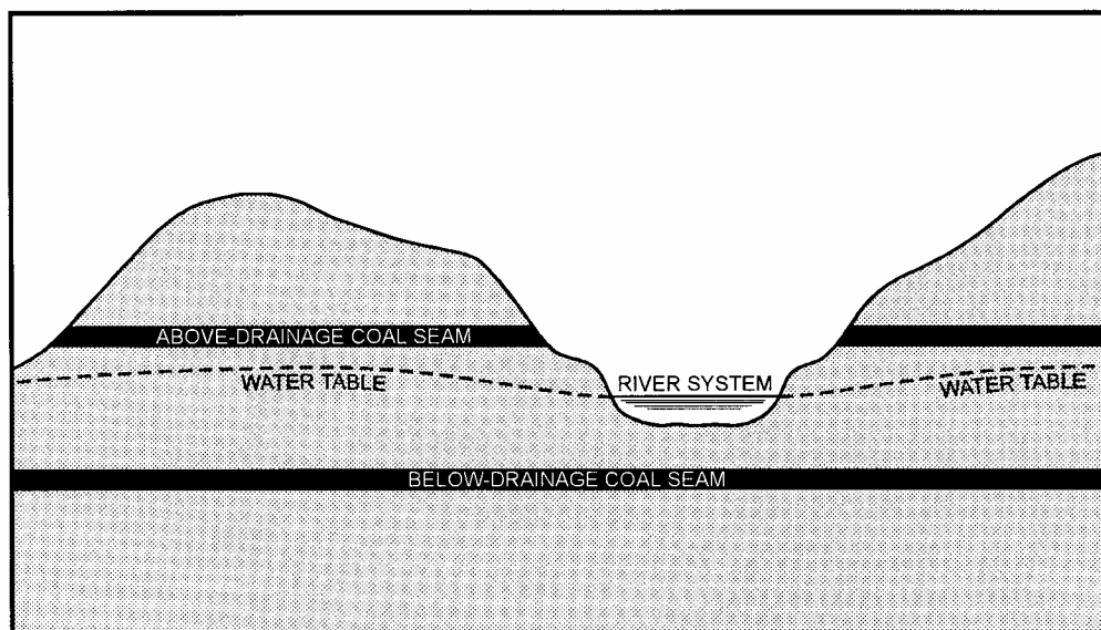
Figure 1. A simplified illustration of underground mines that are distinguished as "below-drainage" or "above-drainage." This refers to their capacity to be completely flooded after abandonment due to their relative location to the regional water table or regional flow system. See Callaghan et al. (1998) for a more thorough and detailed discussion of groundwater flow in the Appalachian Region of the USA.
