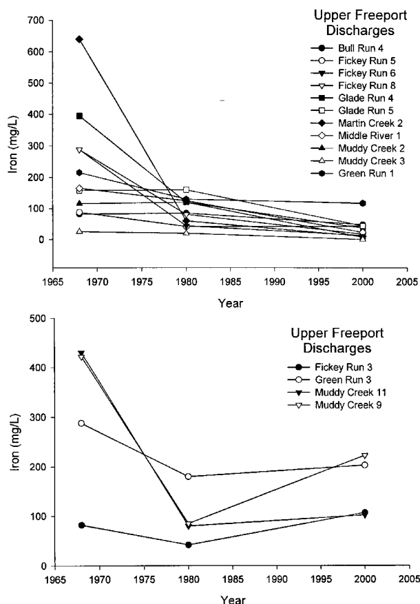
Figure 6. Changes in iron for Upper Freeport sites where we had data for 1968, 1980, and 1999-2000. The top graph shows 11 sites with iron decreases, while four sites showed iron increases.
