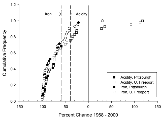
Figure 3. Cumulative frequency plot for acidity and iron for two dates (1968 and 1999–2000). The percent change values of -38.8 for acidity and -59.2 for iron (Table 4) are used as conservative thresholds to indicate that changes more negative than these values are significantly different from a percent change of zero.
