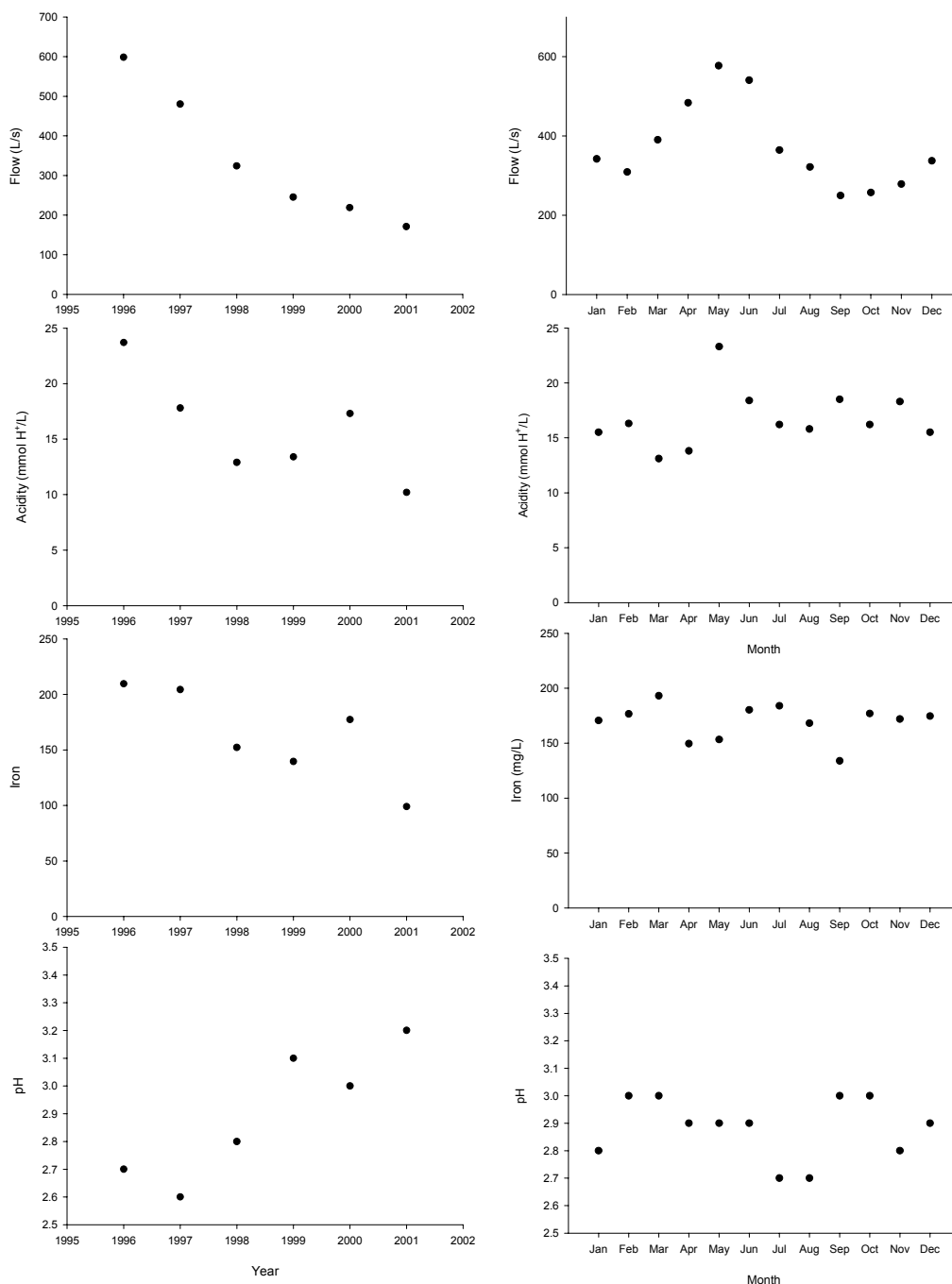
Figure 2. Average values for flow, acidity, iron, and pH across years and months for the T&T data set.
