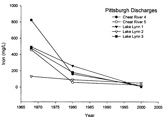
Figure 4. Changes in acidity and iron for five Pittsburgh sites where we had data for 1968, 1980, and 1999–2000. All five sites showed decreasing acidity and iron values.
