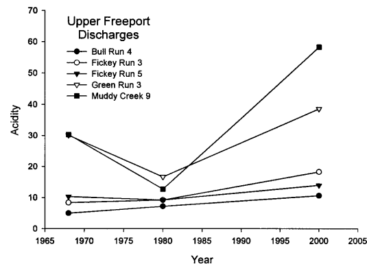
Figure 5. Changes in acidity for Upper Freeport sites where we had data for 1968, 1980, and 1999–2000. The top graph shows 10 sites with acidity decreases, while five sites showed acidity increases.
